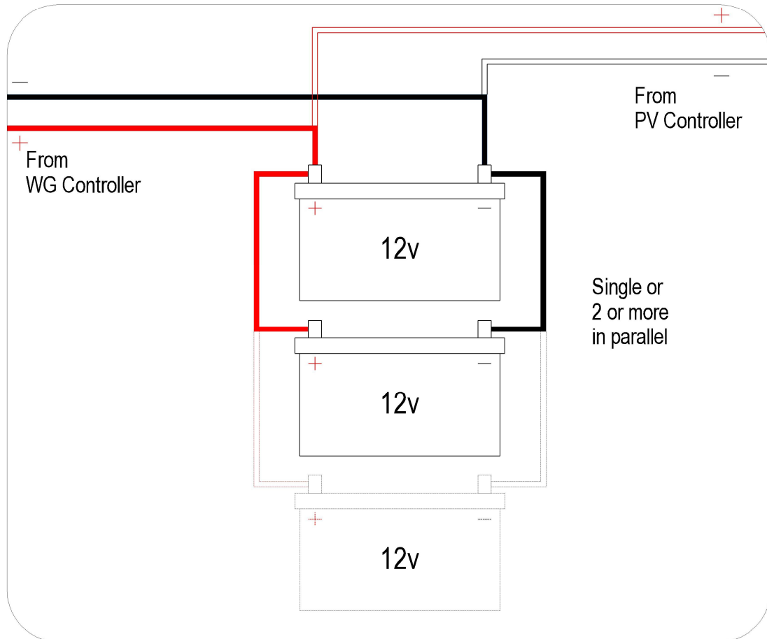
Batteries in Parallel (12v)
