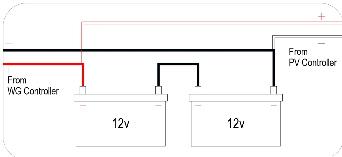
Batteries in Series (24v)
